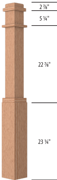
LJ-4391CR Box Newel
