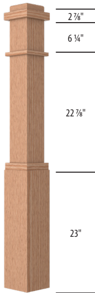
LJ-4091CR Box Newel
